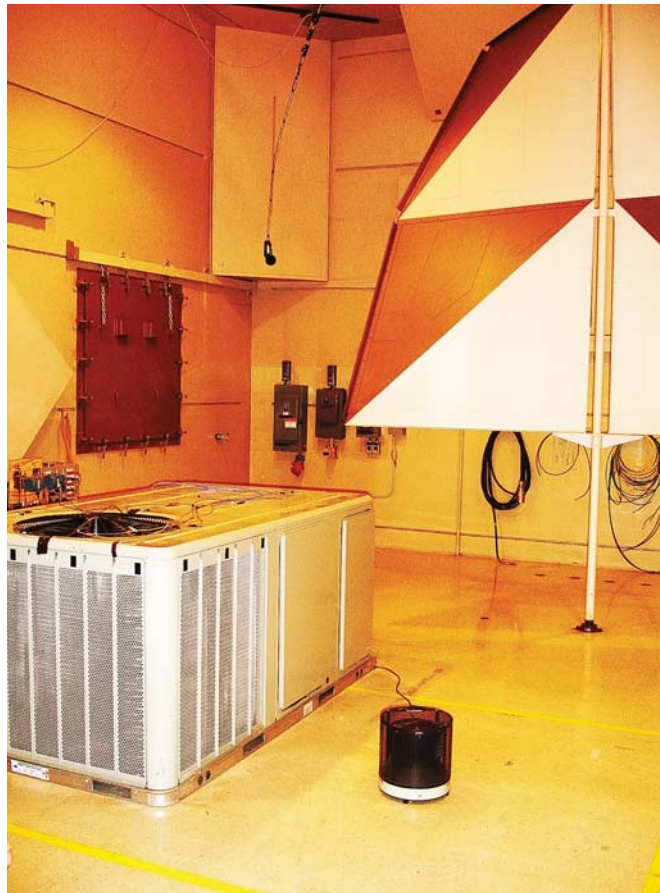
Fig.1. Qualified reverberation room with system ready for sound power measurements.
