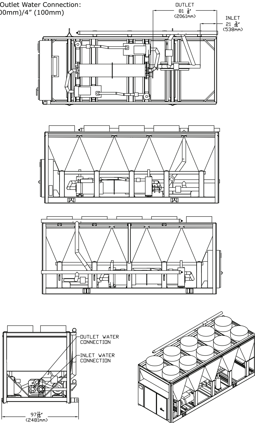
Figure 22. RTAF unit dimensions — 115, 130 ton with free-cooling
