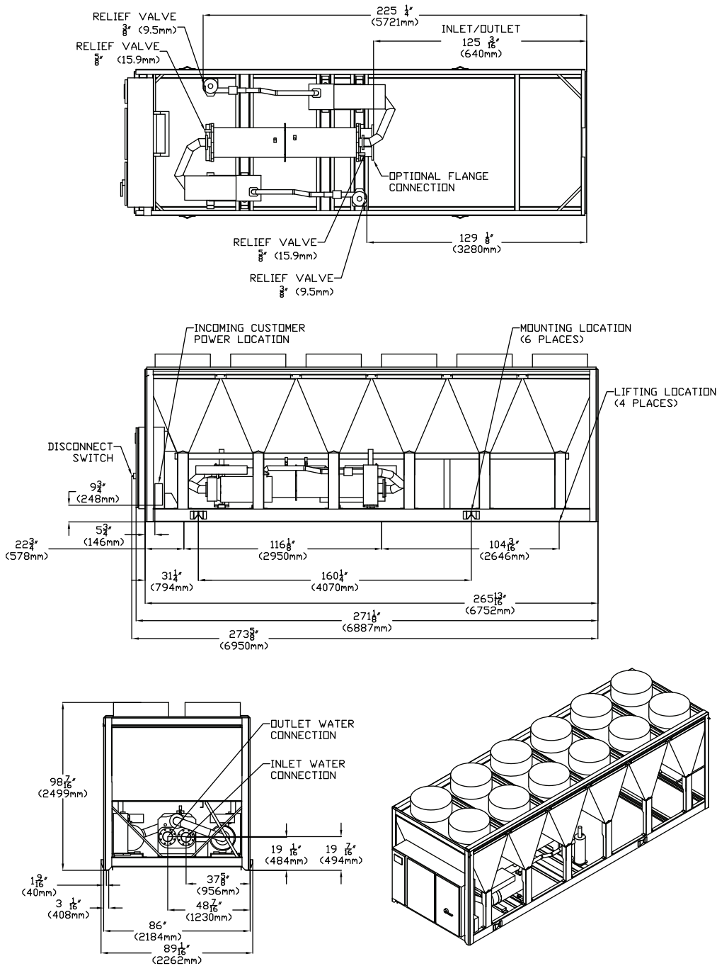
Figure 15. RTAF unit dimensions — 150, 170, 180 ton
