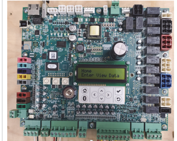
Figure 1. Symbio 700 controller
